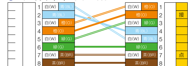
⑩ 110コネクタ(4P)-RJ45 T568B
