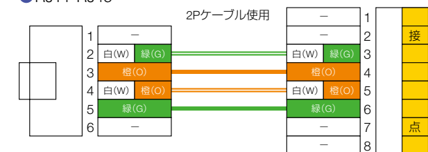
⑫ RJ11-RJ45
