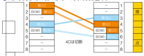
⑪ RJ48 (ISO10173)-RJ45 4C (T568B基準)
